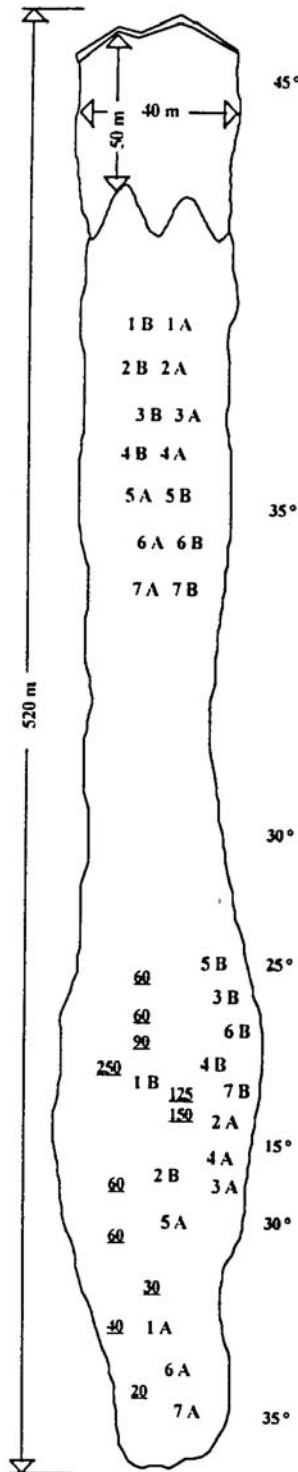
Figure 1: Test avalanche on Rosställispitz (Davos, Switzerland) at 10 March 1996: test configuration, avalanche extent and details on burial of the 14 dummies.
