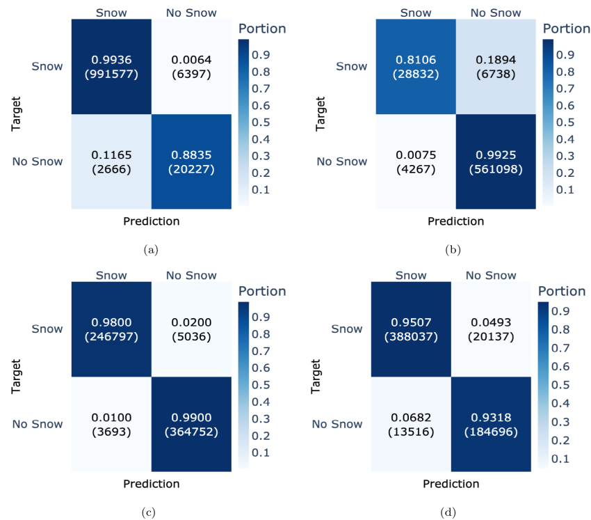
Figure 9. Confusion matrices for each of the four seasonal clusters: (a) winter season (December–April), (b) summer season (July–September), (c) end of the winter season (May–July), and (d) start of the winter season (October–December). Each confusion matrix has targets as rows and predictions as columns.
