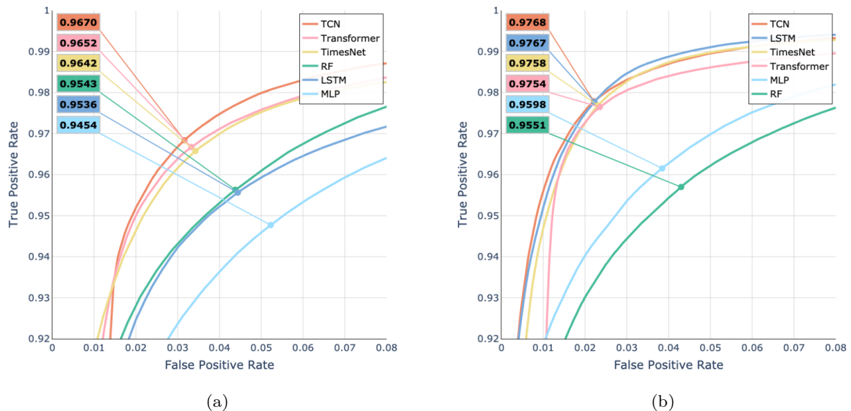
Figure 5. Model comparison shown as ROC curves for two different versions of the six models (LSTM, TCN, TimesNet, transformer, MLP, and RF): model performance with (a) all seven input features (HS, TSS, TA, RSWR, RH, WV, and solar altitude) and (b) the four relevant input features (HS, TSS, TA, and RSWR). Every plot additionally shows the macro-F1 score for the threshold where TPR = FPR (the point on the curve).
