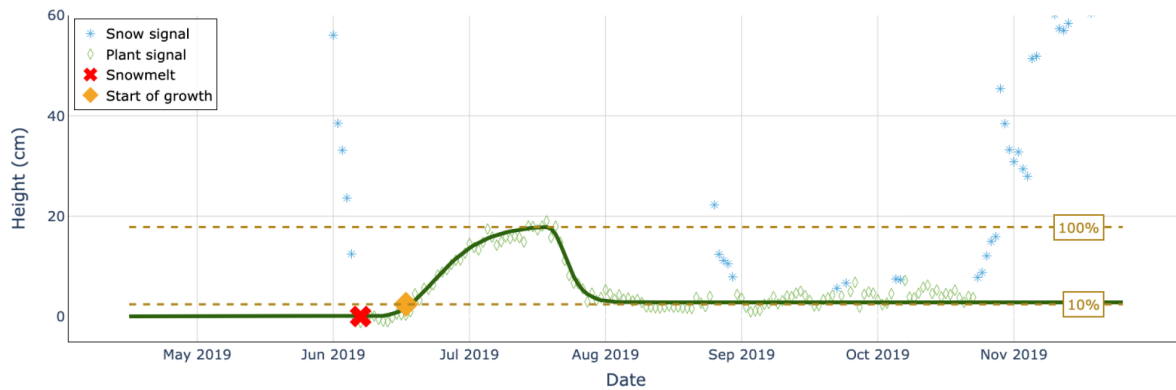
Figure 13. An example of a logistic growth curve (in dark green) fitted to height measurement data from TUJ2 in the vegetation season of the year 2019. Snow height data corresponding to snow are shown with blue stars, while the plant signal is shown with green diamonds. The red cross marks the snowmelt date, while the orange diamond marks the start of plant growth.
