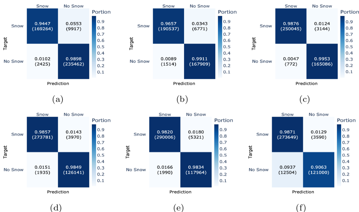
Figure 6. Performance evaluation of each test station separately, shown in terms of confusion matrices ordered by elevation (a–f): SFL2 (1536 m), SHE2 (1852 m), KLO2 (2147 m), TRU2 (2459 m), WFJ2 (2536 m), and STN2 (2914 m). Each confusion matrix has targets as rows and predictions as columns.
