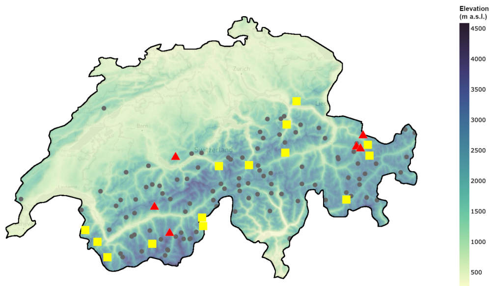
Figure 1. Map of IMIS stations in Switzerland. Stations marked as full gray circles were not part of the new annotated dataset. The yellow squares are the stations that were used for training (14 stations), and the red triangles indicate stations used for testing (6 stations). The background colors indicate the elevation (m a.s.l.).
