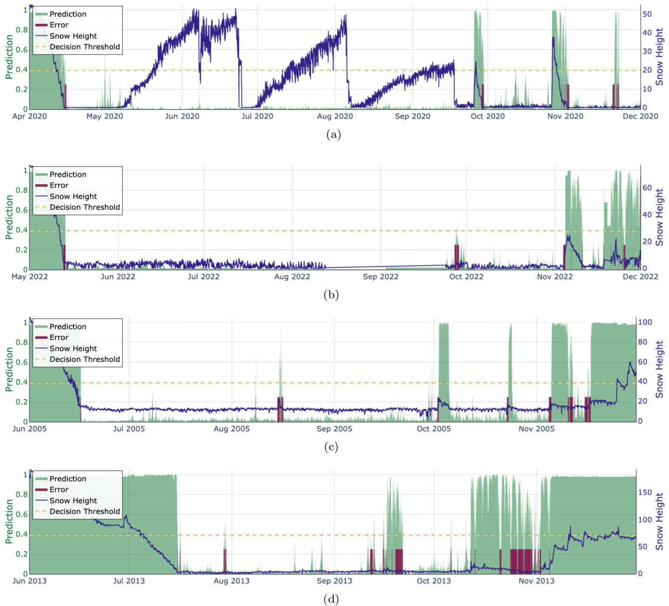
Figure 10. Examples of CleanSnow classification results. The snow height signal is depicted in blue. The model predictions in terms of probability (0–1) are shown in green. The dashed horizontal line denotes the decision threshold selected to balance the model performance in predictions for both classes. The red-shaded areas mark regions with classification errors (i.e., samples assigned to the wrong class). (a) SLF2 (1563 m), year 2020 shows a correct classification of summer vegetation growth (the nonzero blue curve is classified with a probability lower than that of the decision threshold and therefore is assigned to class No Snow). (b) SHE2 (1852 m), year 2022 is an example of early October snowfall that has been classified partially correctly. (c) TRU2 (2459 m), year 2005 demonstrates the model’s ability to detect summer snowfall and scattered snowfall at the beginning of winter. (d) STN2 (2914 m), year 2013 is evidence that the model does not always perform well, here making mistakes at the beginning of the next winter season.
