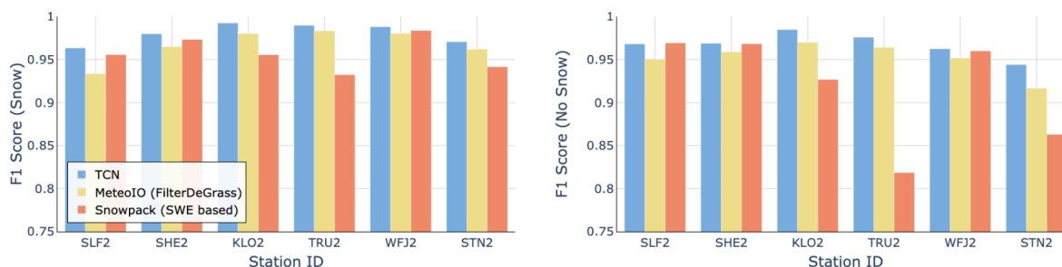
Figure 12. Comparison to other approaches shown as performance (F1 score) per station for CleanSnow (blue), the filter based on the SWE from SNOWPACK (red) and the thresholding filter from MeteoIO (yellow).
