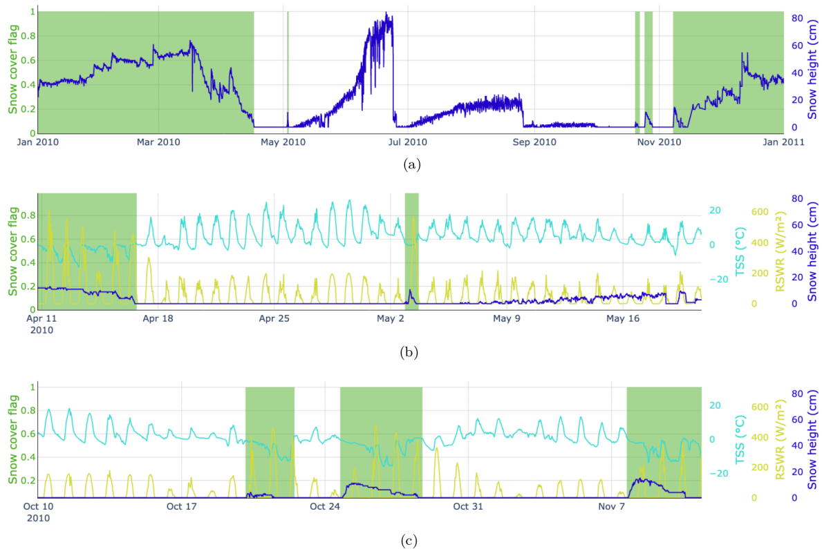
Figure 2. Examples of manually annotated data for the calendar year 2010 at station SLF2. Panel (a) shows the snow cover flag in green (1 for snow cover and 0 otherwise) and the snow height flag in blue for the whole year. Panel (b) focuses on the end of the winter season 2009/10, illustrating the diurnal behavior of TSS and RSWR depending on whether there is snow or not. Panel (c) is the same as panel (b) for the beginning of the winter season 2010/11.
