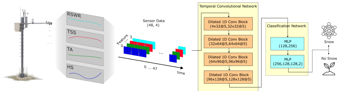
Figure 3. Flowchart of the proposed TCN-based architecture with a drawing of an IMIS station on the left. A time window of four input signals of length 48 (1 d) coming from an IMIS station is fed into the TCN, which causally aggregates information from all the time steps into a 128D latent vector. This information is subsequently fed into the classification network, which applies a sequence of MLPs to classify the input signal into two classes – Snow and No Snow. Each dilated 1D convolutional block has filters described in the format input_features × output_features @ kernel_size . The composition of each MLP is described as input_features , hidden_features_1 , ..., output_features .
