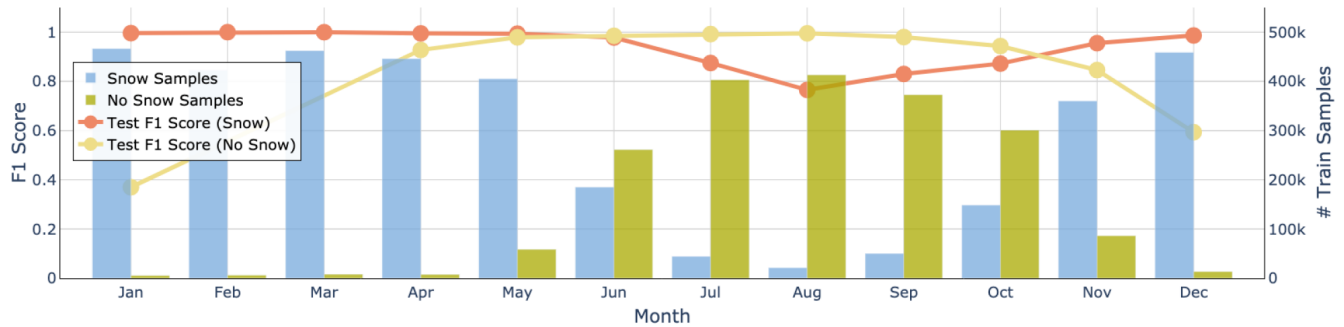
Figure 8. Performance of the model for each month of the year. The F1 score is shown separately for the classifications Snow (red line) and No Snow (yellow line). The blue columns indicate the distribution of the Snow samples, while the yellow columns indicate the distribution of the No Snow samples.
