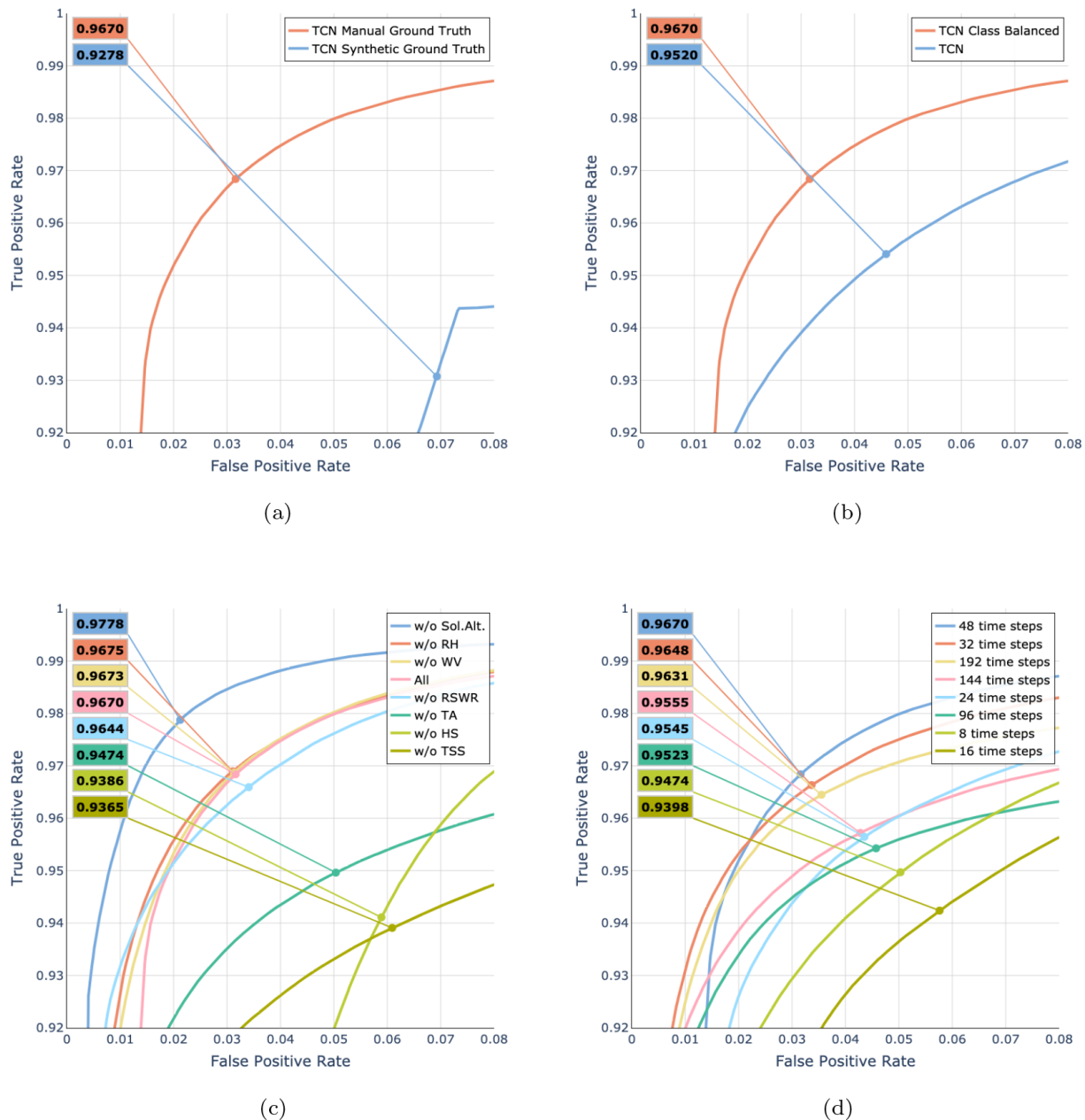
Figure 4. ROC curves for the various ablation studies. Every plot additionally shows the macro-F1 score for the threshold where TPR = FPR (the point on each curve). (a) Importance of manually annotated ground truth data. (b) Effect of class balancing. (c) Importance of input features. (d) Influence of sequence length on model performance.
