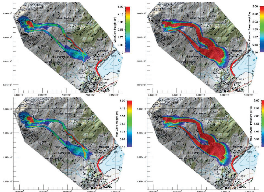
Figure 4: Non-critical simulations for the d_0 = 80 cm scenario. Avalanches stop above the road for warm snow covers (for both deep and shallow snow covers). Secondary releases make the warm, deep snow cover scenario critical.
