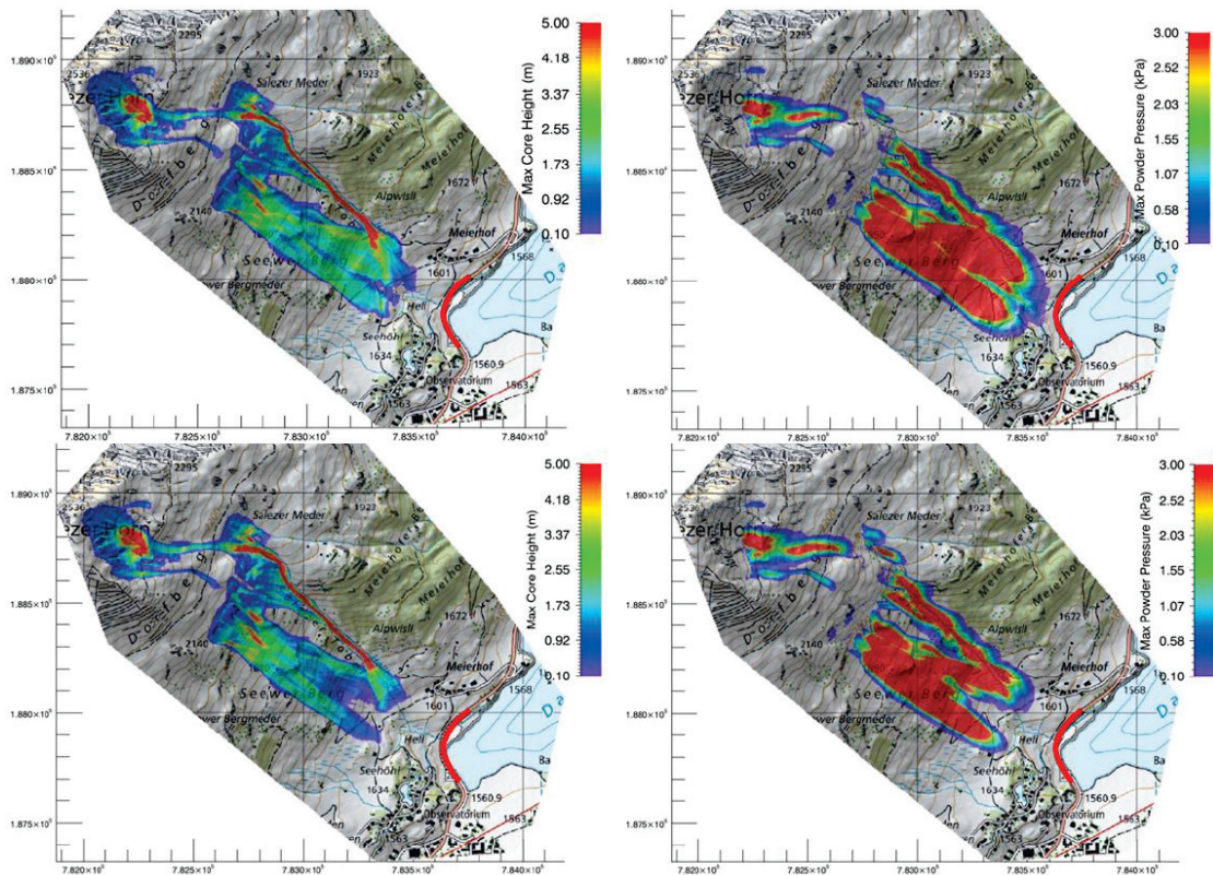
Figure 3: Examples of non-critical simulations for the d_0 = 60 cm scenario. Top: Warm, deep snow conditions, including secondary releases. Bottom: Cold, shallow snow cover, including secondary releases. Both scenarios stopped above the road (including powder cloud).
