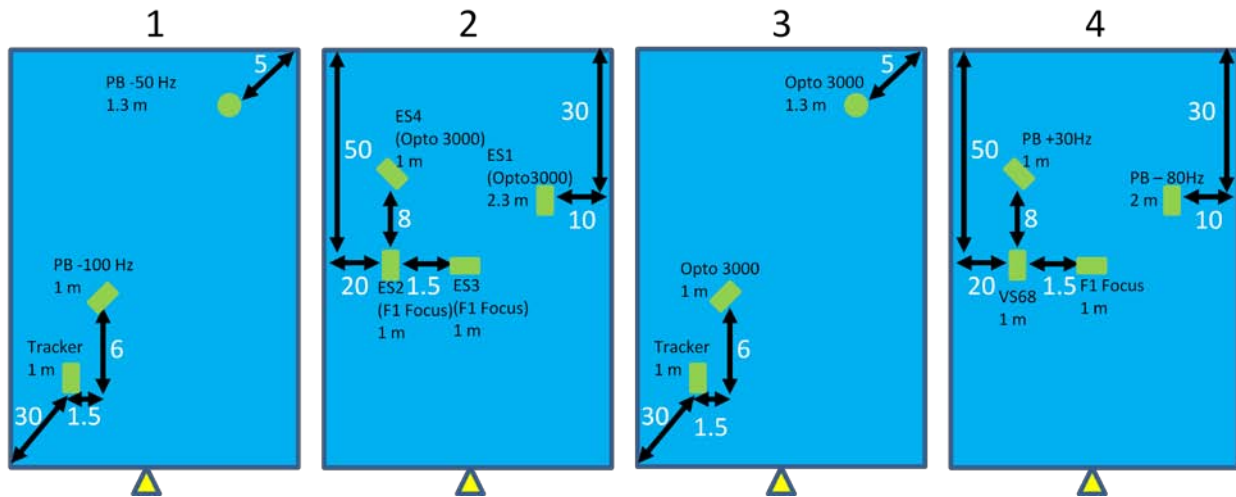
Figure 2: Search scenarios in the test on Col du Lautaret. Same presentation as in Figure 1. All transmitters are turned on at all times. The circular transmitter symbol indicates vertical antenna orientation.
