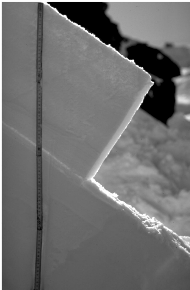
Figure 2. Snowpack configuration at the crown of a slab avalanche: cohesive slab on top of a thin weak layer (buried surface hoar crystals).
