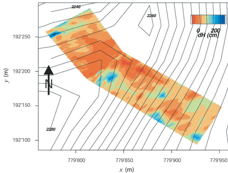
Figure 7. Snow distribution on windward and lee slopes of a mountain ridge with 5-m contour lines (Gaudergrat, near Davos, Switzerland) after a snowdrift period (26–31 January 1999). Main wind direction was northwest. The difference in snow depth dH compared to the snow depth prior to the snowdrift episode is shown. Negative values of dH indicate erosion [from Doorschot et al., 2001] (reprinted from the Annals of Glaciology with permission of the International Glaciological Society).
