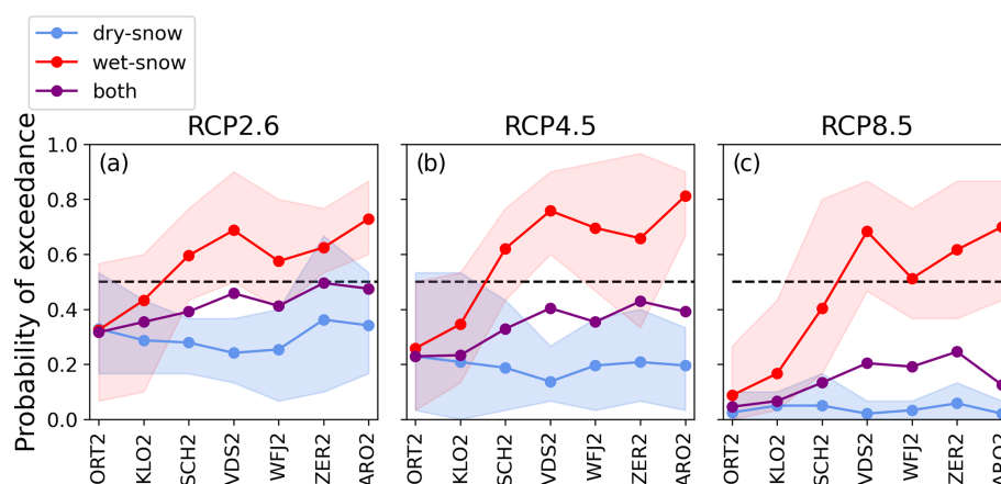
Figure 6. Fraction of seasons in the EOC period (2070–2099) that exceeds the median number of AvDs per season (DJFMAM) in the REF period regarding dry-snow (blue), wet-snow (red), and dry- or wet-snow avalanche activity (purple) for the seven stations and different emission scenarios (RCP2.6 a , RCP4.5 b , and RCP8.5 c ). The markers show the multi-model mean, and the shaded areas correspond to the full model spread. Markers between individual stations are connected for illustration purposes. Stations are arranged in order of increasing elevation, from the lowest (ORT2, 1824 m a.s.l.) to the highest (ARO2, 2847 m a.s.l.).
