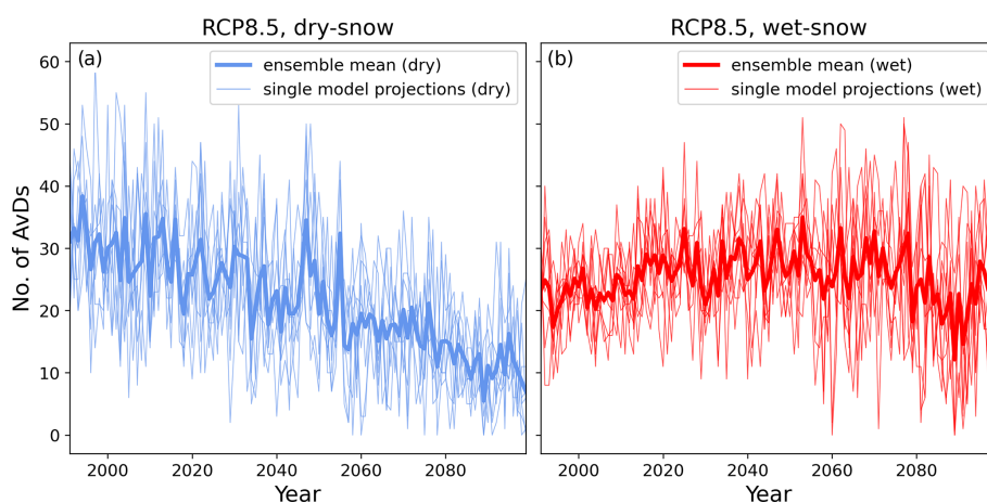
Figure D3. Projected number of (a) dry-snow and (b) wet-snow AvDs for the station WFJ2 (2540 m a.s.l.) at a yearly resolution for the time span 1991–2099. The thin lines indicate projections by individual model chains, and the bold line shows the multi-model mean.
