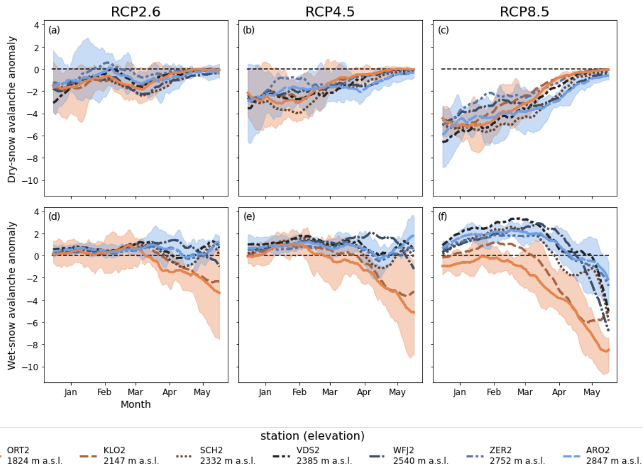
Figure D1. Mean monthly dry- and wet-snow avalanche anomaly for the 2070–2099 period compared to the 1991–2020 period for RCP2.6 (a, d), RCP4.5 (b, e), and RCP8.5 (c, f). The lines show the multi-model mean for seven AWSs across the Swiss Alps. The shaded areas indicate the spread of the eight ensemble members for the highest and lowest AWSs. Station identification is facilitated by colors and line styles specified in the bottom legend.
