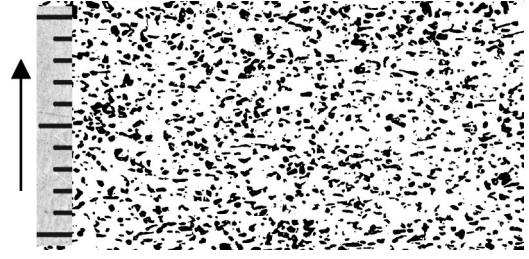
FIG. 3. Microstructure of snow type tested. Binarized picture of a surface section. Black denotes ice, white is the pore space ( \rho = 250 \text{ kg m}^{-3} ). Scale given is 1 cm. Arrow points to the snow surface (top margin was parallel to the snow surface).
