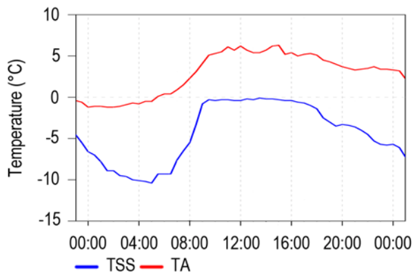
Figure 2: Meteorological conditions for 28 April 2010: air temperature (TA, red) and snow surface temperature (TSS, blue).
