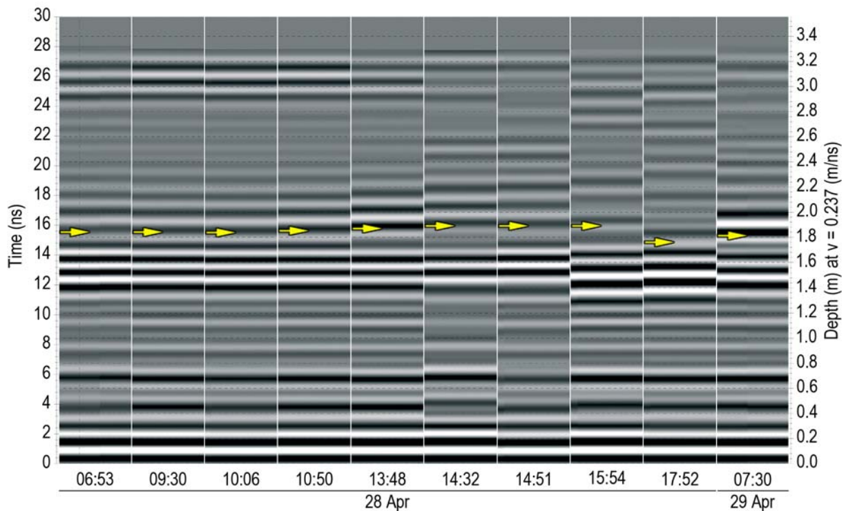
Figure 3: Radargram for 28 April 2010. The left ordinate displays the TWT in ns and the right ordinate shows the calculated snow height utilizing a mean wave speed of \bar{v} = 0.237 m/ns. The yellow arrows indicate the snow surface reflection.
