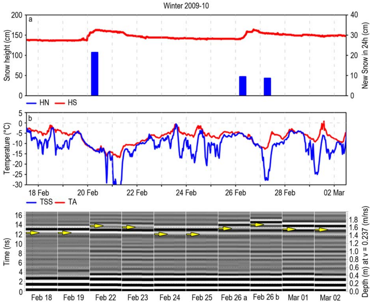
Figure 1: Meteorological conditions and radargrams for the period 18 February - 3 March 2010. (a) snow height (HS, red) and amount of new snow (HN24, blue), (b) air temperature (TA, red) and snow surface temperature (TSS, blue), (c) corresponding radargrams; the left ordinate displays the TWT in ns and the right ordinate shows the calculated snow height utilizing a mean wave speed of \bar{v} = 0.237 m/ns. The yellow arrows indicate the snow surface reflection.
