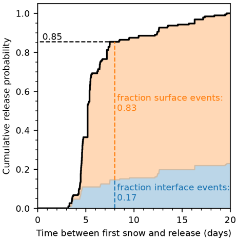
Figure C1. Cumulative release probability for 20 d after the first snowfall on snow-free ground. The avalanches were classified into surface (orange) and interface (blue) events.
