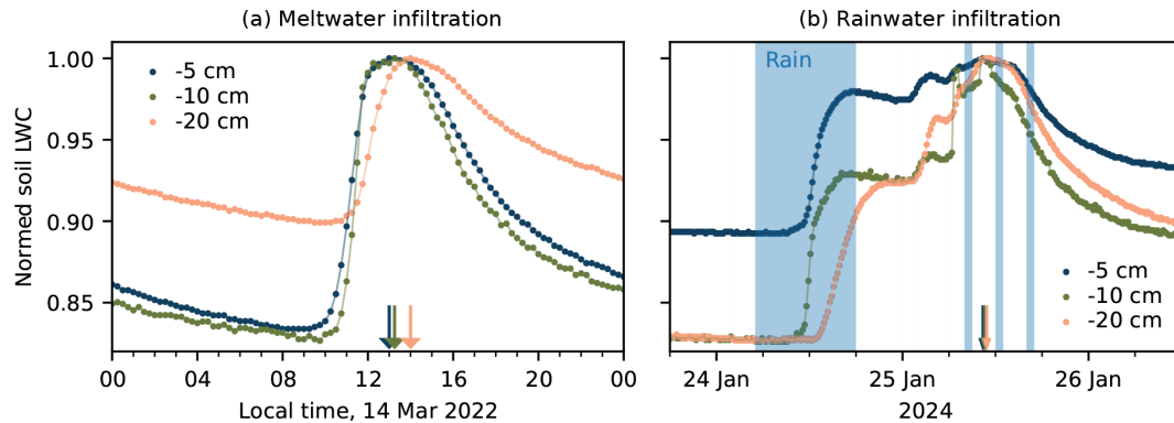
Figure 8. Normalized LWC for three soil depths which show (a) meltwater and (b) rainwater infiltration. The soil LWC was normalized with the maximum value to better visualize the time shift in the percolation. The arrows indicate the time of the maximum. The time of rain (blue) was extracted from the SNOWPACK simulation at the reference location.
