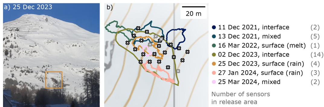
Figure 4. (a) Picture of the release area on the Seewer Berg slope (rectangle) on 25 December 2023. (b) Release areas extracted from time-lapse photographs for glide-snow avalanches on the sensor grid. Every avalanche was classified based on the source of interfacial water: interface (water originated from the soil–snow interface), surface (water originated from the snow surface), and mixed (combined interface and surface). Grid sensors (×) that were not used for soil LWC observations are marked in gray. The number of sensors within the release area after manual modification (without excluded gray sensors) is given in parentheses for every avalanche. Map: Federal Office of Topography, north up, contour line spacing of 10 m.
