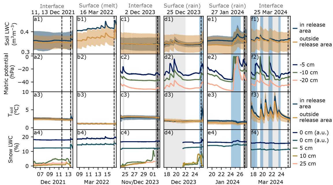
Figure 6. (a–f) Soil and snow measurements throughout the 8 d before avalanche release. The background color indicates patchy (gray) or continuous (white) snow cover or rain (blue). The dashed line indicates the time of avalanche release on the Seewer Berg slope with the range of uncertainty in dark gray. Results from sensor groups (inside/outside the release area) are visualized as the mean (line) and standard deviation (shading) between the sensors within the group. The parameters include the following: (a1–f1) the soil LWC for sensors located inside (blue) and outside (yellow) the release area. (a2–f2) The soil matric potential which has been recorded since summer 2022. (a3–f3) The soil temperature inside (blue) and outside (yellow) the release area. (a4–f4) The snow LWC sensors at the interface (arbitrary units) and at three snow heights. When there are no measurements available (b4, e4, f4), this was due to insufficient snow heights which caused preferential melt around the wedges.
