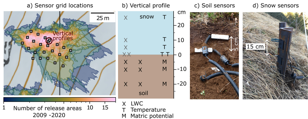
Figure 3. (a) The Seewer Berg slope with the location of the soil LWC sensors (×). The maroon circle indicates the location of the vertical profiles across the soil–snow interface. (b) Schematic of the vertical soil–snow profile. The soil LWC sensors and matric potential sensors have an integrated temperature sensor. (c) Picture of a vertical soil LWC profile. (d) Picture of the wedges for snow LWC and temperature monitoring. Map: Federal Office of Topography, north up, contour line spacing of 10 m.
