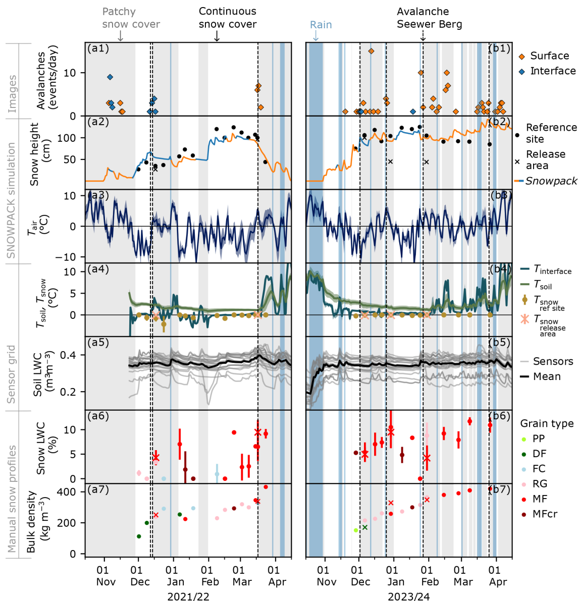
Figure 5. Overview (daily mean values) of (a) season 2022 and (b) season 2024. The background colors indicate patchy snow cover (gray), continuous snow cover (white), or rain (blue). The dashed line indicates the time of avalanche release on the Seewer Berg slope. (a1, b1) Avalanche activity on Dorfberg derived from time-lapse photographs classified as surface (orange) or interface (blue) events based on the SNOWPACK simulation. (a2, b2) Snow height simulated at the reference location (line, classified as surface/interface with SNOWPACK) and snow heights from manual snow profiles at the reference location (·) or from avalanches on the Seewer Berg slope (×). (a3, b3) Air temperature at the reference location (SNOWPACK). (a4, b4) Mean soil temperature across the sensor grid, the mean interface temperature, and the interfacial snow temperature from the manual snow profiles. (a5, b5) Soil LWC recorded by the individual sensors (gray) and the mean across all grid sensors (black). (a6, b6) Snow LWC observed in the manual snow profiles in the reference location (·) and behind the fracture line of avalanches on the Seewer Berg slope (×). The color indicates the grain type of the lowermost snow layer. (a7, b7) Snowpack bulk density colored by the dominant grain type within the snow profile. Grain types: precipitation particles (PP), decomposing and fragmented precipitation particles (DF), faceted crystals (FC), rounded grains (RG), melt forms (MF), melt–freeze crust (MFcr).
