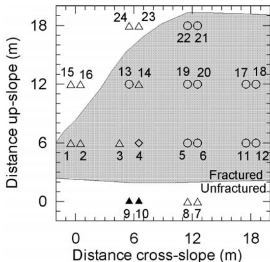
Figure 1. Rammrutsch sampling locations at the Swiss site, with the numbers indicating the test order. Gray area indicates the assumed extent of the fracture within the study area. Open triangles represent points not used in the analysis because they did not fracture on the targeted weak layer. Solid triangles represent points where the fracture occurred in the targeted weak layer, but are located outside our assumed weak layer collapse area. The diamond represents the test prior to the collapse, and the circles are post-collapse data points.
