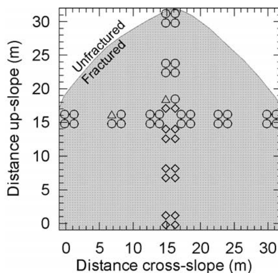
Figure 2. Shear frame test locations at our Montana site. Gray area indicates the assumed extent of the fracture within the study area. Diamonds indicate samples taken before the collapse, circles show the post-collapse measurements, and the two triangles represent outliers not considered in the calculation of the sintering rate (see Figure 4).
