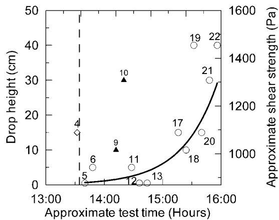
Figure 3. Rammrutsch drop height plotted versus approximate test time shows an increasing strengthening rate of the weak layer. The collapse occurred at the vertical dashed line. Same symbols as in Figure 1.
