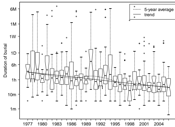
Figure 6: Burial time of completely buried persons found without visible parts.
