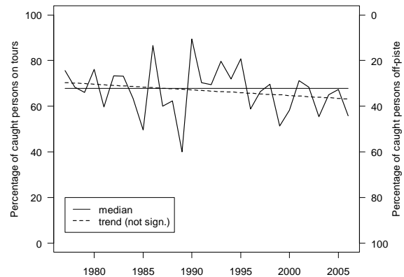
Figure 3: Ratio of people caught on ski tours to people caught in off-piste terrain. There is a marginal trend to more off-piste accidents, which is not significant.
