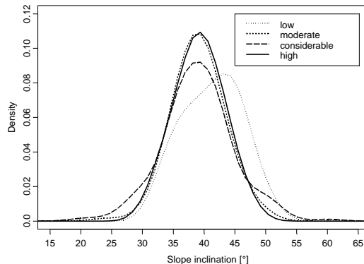
Figure 12: Density of slope inclination of recreational avalanche accident for the avalanche danger degree “low” to “high”. The steepest part of the slope of recreational avalanche accidents is for all danger degrees roughly the same. However the trigger probability and the distribution of danger spots are different for each danger degree.
