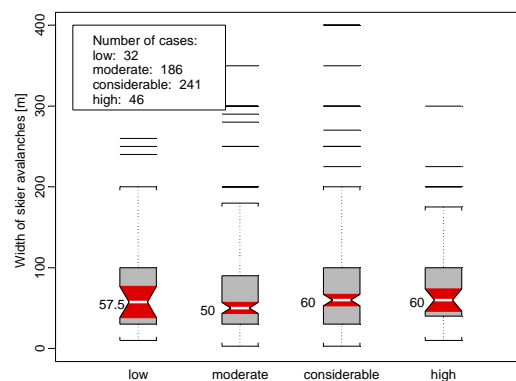
Figure 9: Width of recreational avalanche accidents 1988 to 1999 (12 years).
