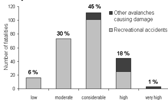
Figure 3: Number of fatalities for each danger degree during the period between the winters 1987/88 and 1998/99. Total number of fatalities during the forecasting periods: 248 (Recreational accidents: 215, others: 33).
