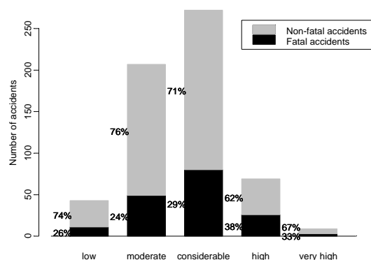
Figure 4: Avalanches causing damage to people 1988 to 1999 (12 years).
