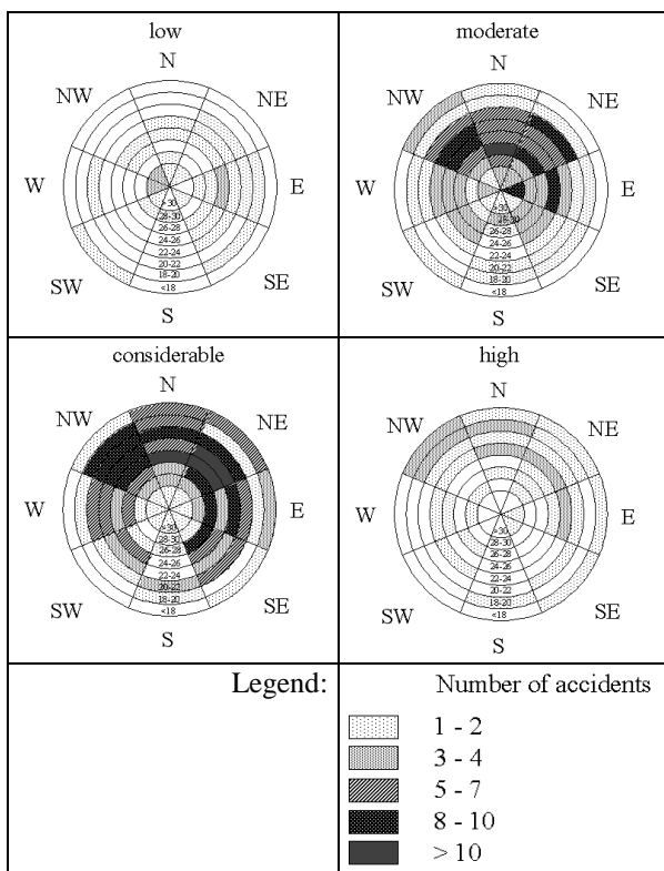
Figure 11: Aspect and altitude for recreational avalanche accident at each danger degree 1988 to 1999 (12 years). (The altitudinal belts are specified in 100 m steps: e.g. 22 correspond to 2200 m a.s.l.). Total number of cases considered: 575
