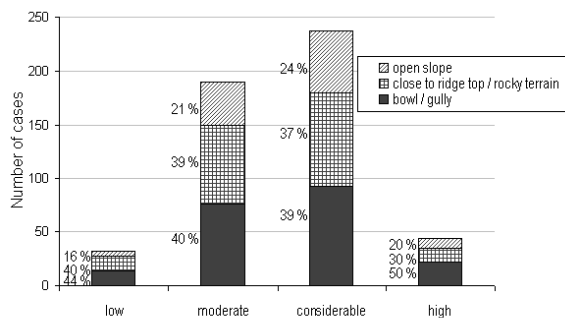
Figure 13: Frequency of slope shapes for each danger degree.
