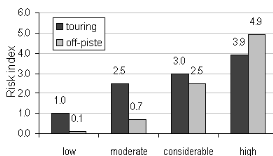
Figure 16: Risk index for damage to people doing winter sport on tours and off-piste. For comparison the touring-risk-index for degree low was set to one and the other indices were adapted accordingly.
